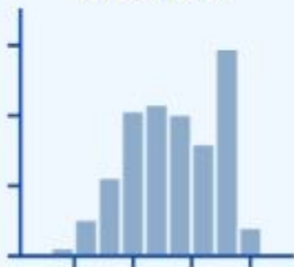
Histogram
