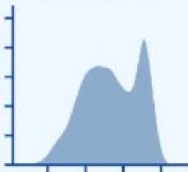
Density Plot
